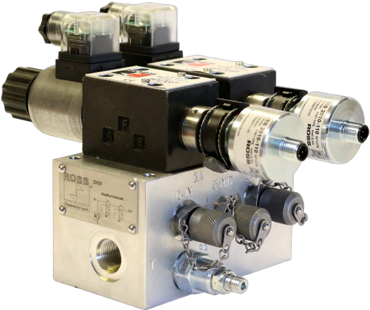
ROSS® HBB Series Valve System for Block & Bleed
